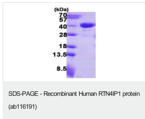
15% SDS-PAGE analysis of 3 µg ab116191.
