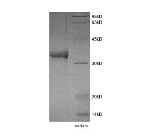
SDS-PAGE - Recombinant Human PR3 protein (ab153798)
