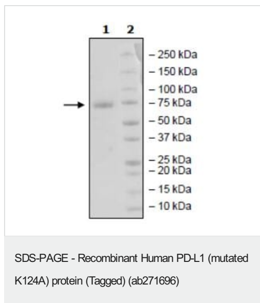
SDS-PAGE analysis of ab271696.
