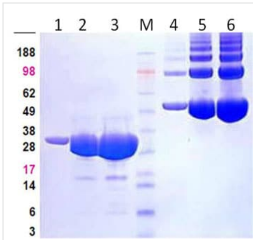
SDS-PAGE analysis of PAK2 (ab95310) and BSA
