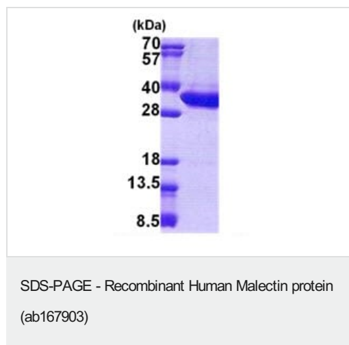
15% SDS-PAGE analysis of ab167903 (3µg).
