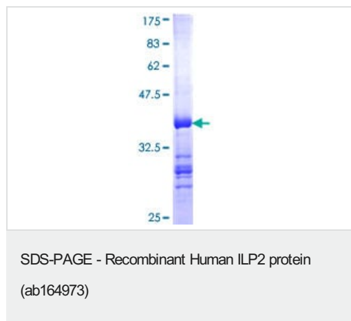
ab164973 on a 12.5% SDS-PAGE stained with Coomassie Blue.
