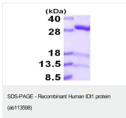
15% SDS-PAGE analysis of ab113598 (3µg)
