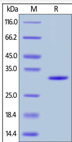
SDS-PAGE - Recombinant human Galectin 3 protein (ab179972)
