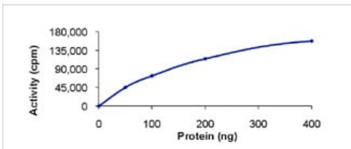
Functional Studies - Recombinant human FIST protein (ab85601)
