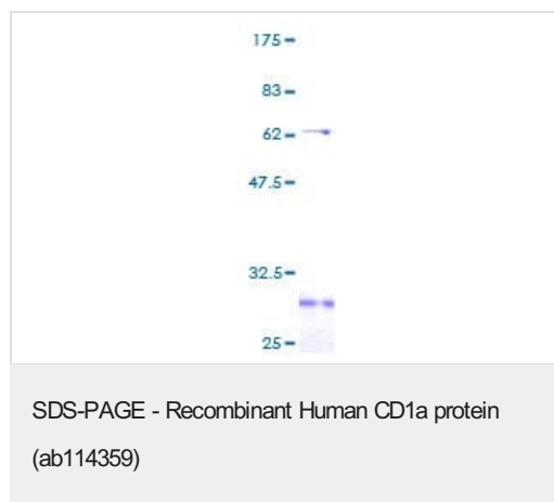
12.5% SDS-PAGE showing ab114359 at approximately 59.95kDa stained with Coomassie Blue.
