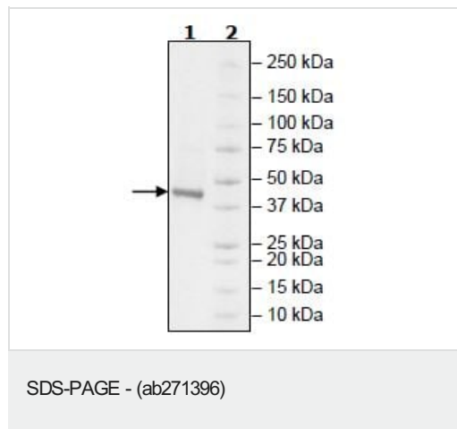
SDS-PAGE analysis of ab271396.
