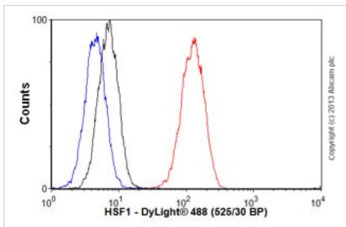
Flow Cytometry - Anti-HSF1 antibody [10H8] (ab61382)
