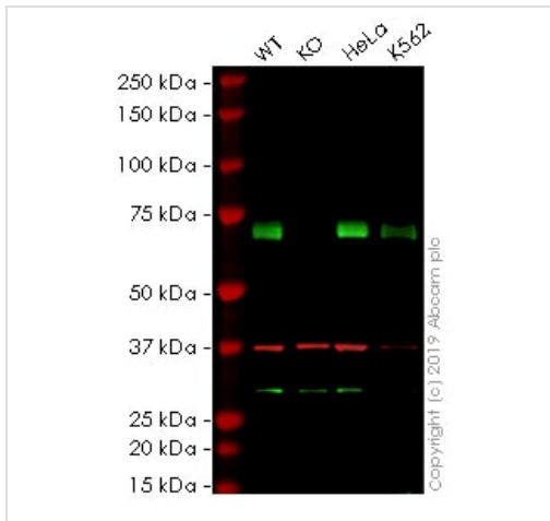
Western blot - Anti-HSF1 antibody [10H8] (ab61382)
