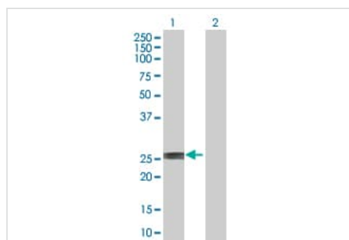
Western blot - RERG overexpression 293T lysate (whole cell) (ab94205)
