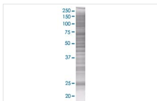
SDS-PAGE - RERG overexpression 293T lysate (whole cell) (ab94205)
