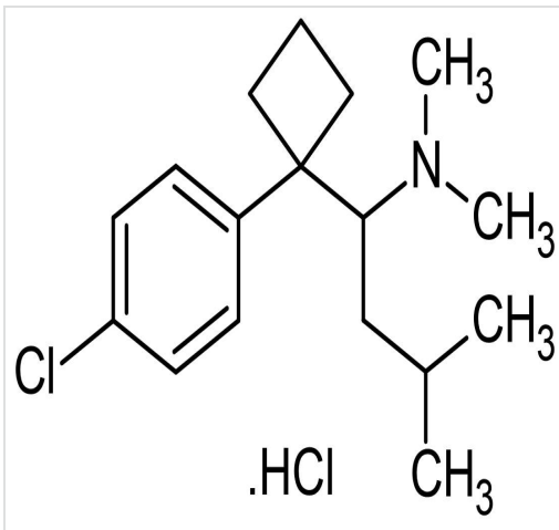
Chemical Structure - Sibutramine hydrochloride, Serotonin, Noradrenaline and Dopamine reuptake inhibitor (ab120529)
