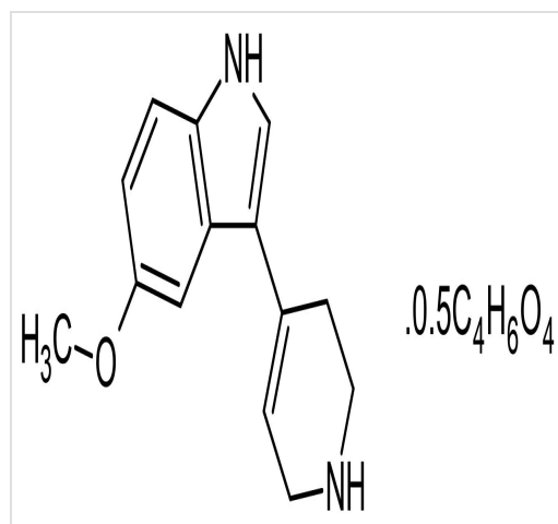
2D chemical structure image of ab146299, RU 24969 hemisuccinate, 5-HT1A/1B agonist
