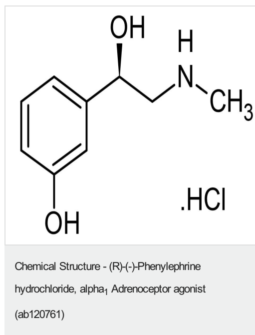
2D chemical structure image of ab120761, (R)-(-)-Phenylephrine hydrochloride, \alpha_1 Adrenoceptor agonist
