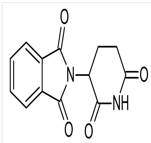
Chemical Structure - (±)-Thalidomide, Immunomodulator and anticancer agent (ab120032)
