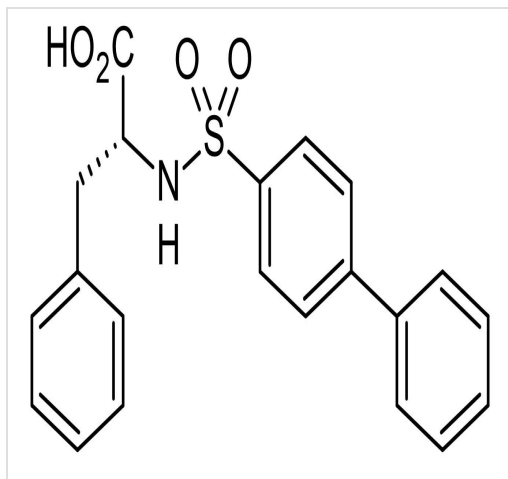
Chemical Structure - MMP-2/MMP-9 Inhibitor I, MMP-2/MMP-9 inhibitor (ab145190)
