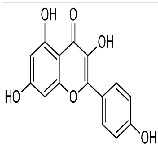
Chemical Structure - Kaempferol, Phytoestrogen (ab120357)
