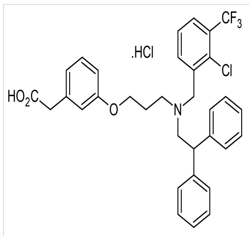
2D chemical structure image of ab141299, GW 3965 hydrochloride, LXR agonist
