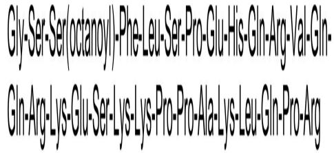
Chemical Structure - Ghrelin (human), Endogenous GHS agonist (ab120230)
