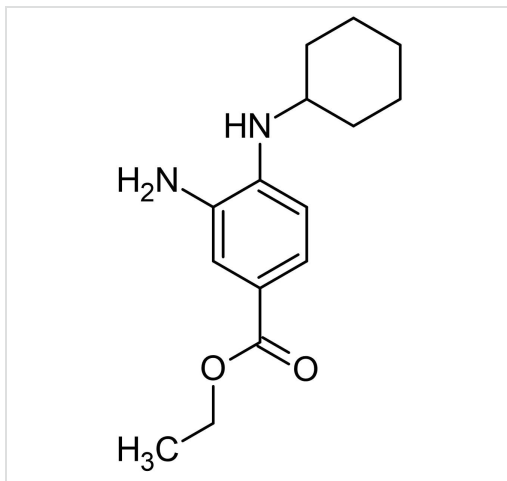
Chemical Structure - Ferrostatin 1, erastin-induced ferroptosis inhibitor (ab146169)
