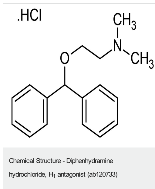
2D chemical structure image of ab120733, Diphenhydramine hydrochloride, H 1 antagonist
