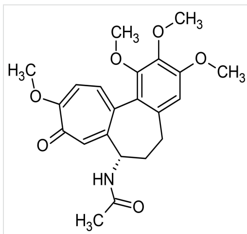
Chemical Structure - Colchicine from Colchicum autumnale , microtubule formation inhibitor (ab120663)
