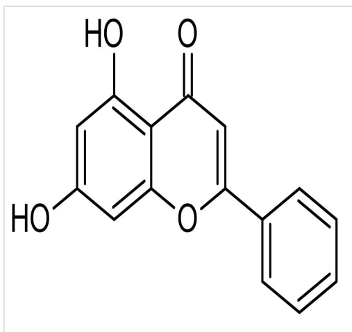
Chemical Structure - Chrysin, Antioxidant flavonoid (ab141230)
