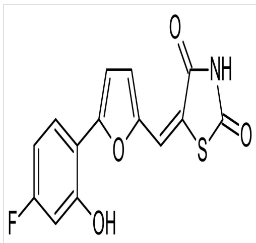
Chemical Structure - AS-252424, PI3Kgamma inhibitor (ab120929)
