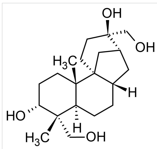
Chemical Structure - Aphidicolin, DNA polymerase alpha, delta and epsilon inhibitor (ab142400)
