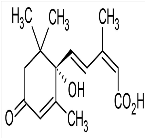
Chemical Structure - (+)-Abscisic acid, Phytohormone (ab120860)
