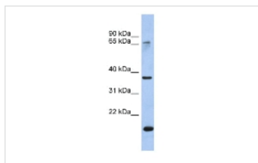
Western blot - Anti-Annexin A10 antibody (ab95091)
