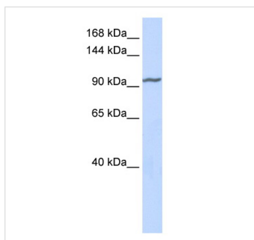
Western blot - Anti-ZNF280D antibody (ab85881)
