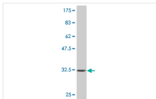
Western blot - Anti-INPP4B antibody (ab76477)
