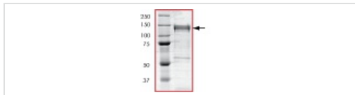
ab60754 on SDS-PAGE, MW ~130kDa.
