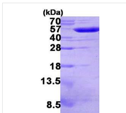
SDS-PAGE - Recombinant E. coli gor protein (ab123214)
