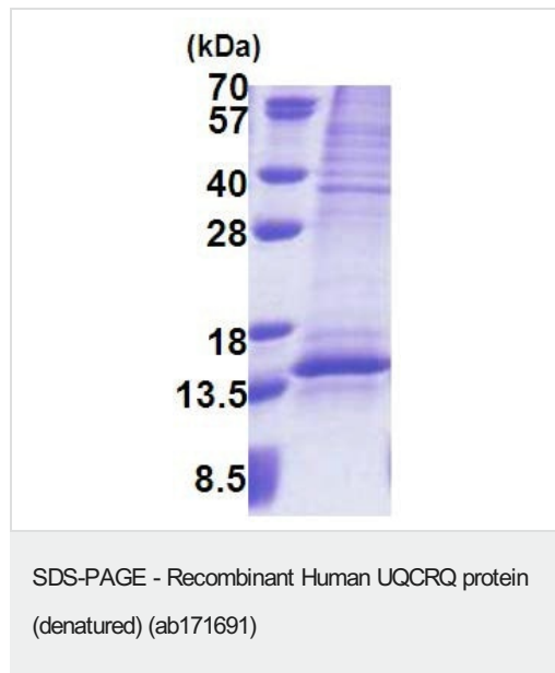
15% SDS-PAGE analysis of ab171691 (3 \mu g).
