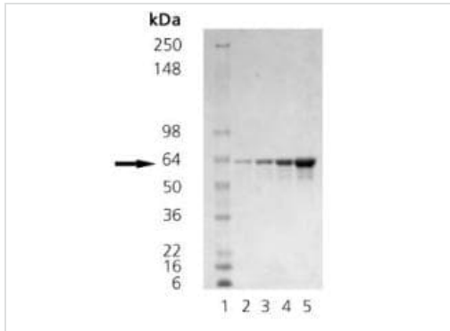
SDS-PAGE - Recombinant Human STIP1/STI1 protein (ab92357)
