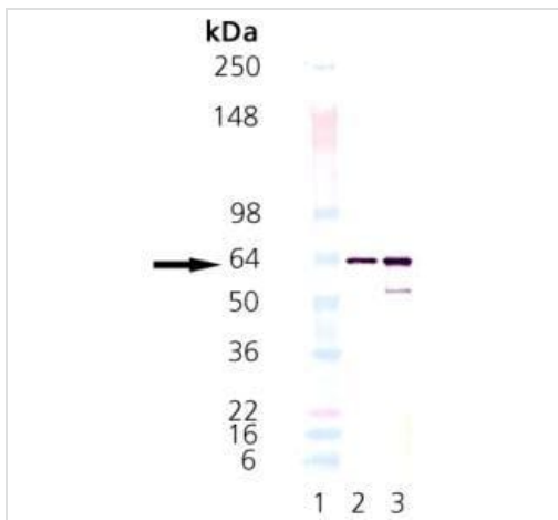
Western blot - Recombinant Human STIP1/STI1 protein (ab92357)
