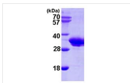
15% SDS-PAGE analysis of 3 µg ab102020.
