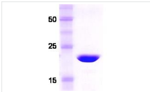
SDS-PAGE - Recombinant Human Recoverin protein (ab48757)
