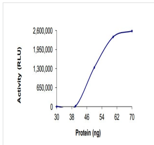
Functional Studies - Recombinant human PDE4C protein (ab125647)
