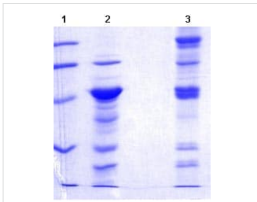
SDS-PAGE - Recombinant Human NUCB2 protein (ab101042)
