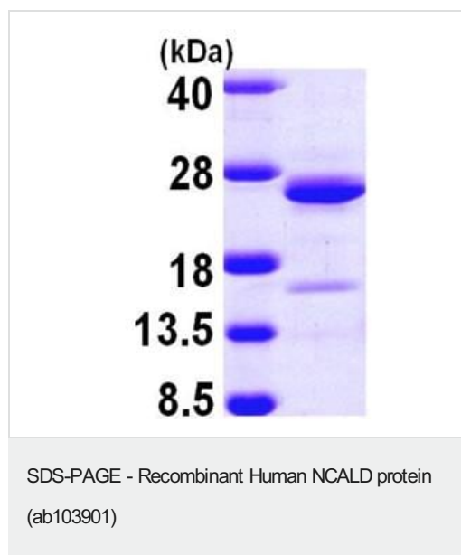
15% SDS Page analysis of ab103901 (3 µg)
