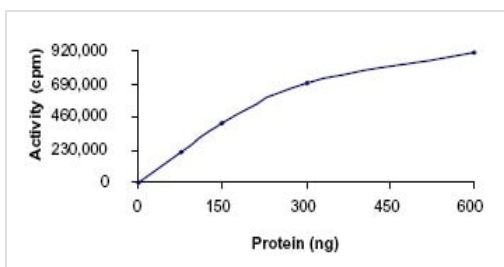
IRR enzymatic activity.
