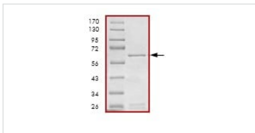
SDS page analysis of ab69988
