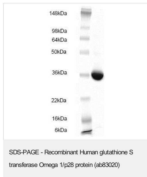
SDS-PAGE showing ab83020 at approximately 28kDa.
