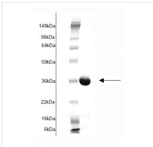
ab82954 on SDS-PAGE.
