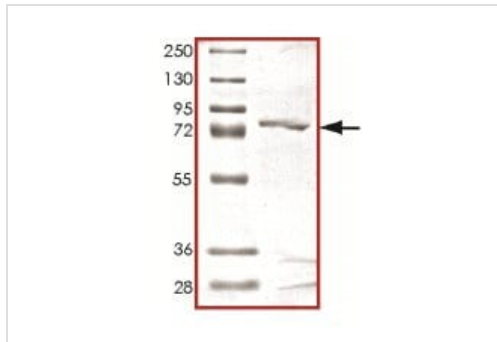
SDS-PAGE analysis of ab125570.
