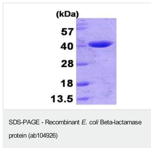
15% SDS-PAGE analysis of 3ug ab104926
