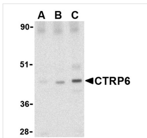
Western blot - Anti-CTRP6 antibody (ab36900)
