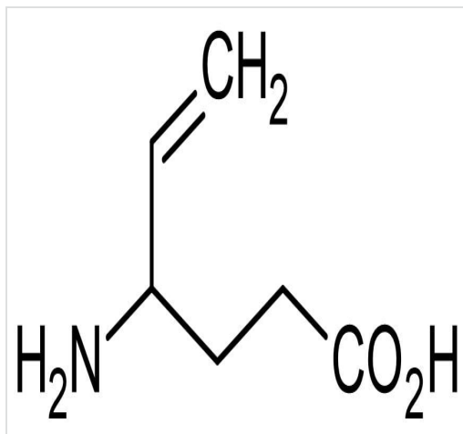
Chemical Structure - Vigabatrin, Irreversible GABA transaminase inhibitor (ab120310)
