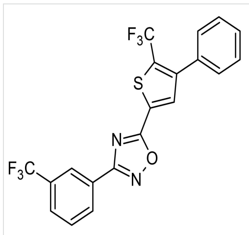
2D chemical structure image of ab120983, SEW 2871, S1P1 agonist
