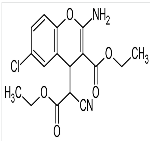
Chemical Structure - SC79, Akt activator (ab146428)
