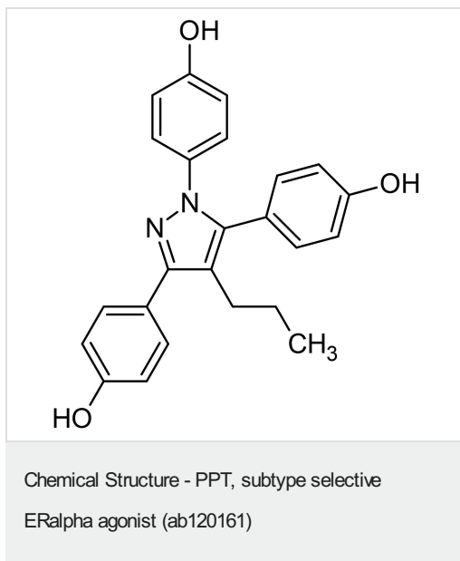
2D chemical structure image of ab120161, PPT, subtype selective ERalpha agonist
